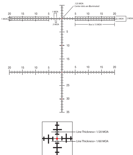
Close-Up of Center Crosshairs at 0 MOA and 20 MOA
